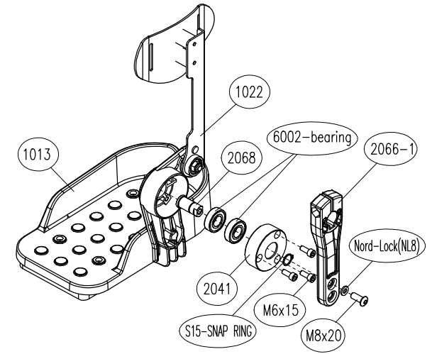
Pedal-R assemble
